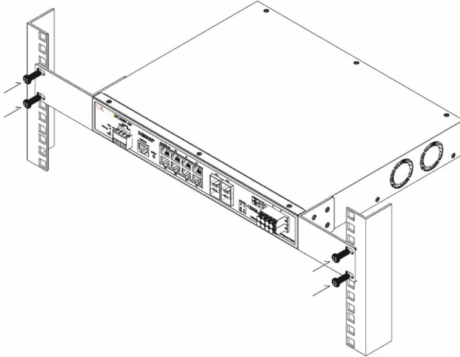
SFC410BT Series Rack Mount 장착 모습
