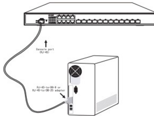
Figure 3-5 Connecting the console port of SFC4200A and computer
