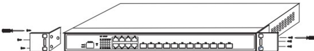
Figure 3-1 Fixing the machine box of the switch
