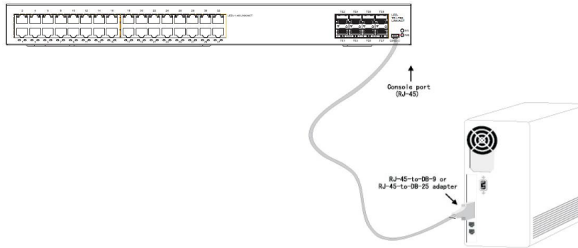
Figure 3-5 Connecting the console port of SFC5540T and computer
