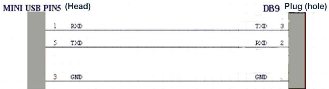
Figure 3-4 Cable connection at the console port
