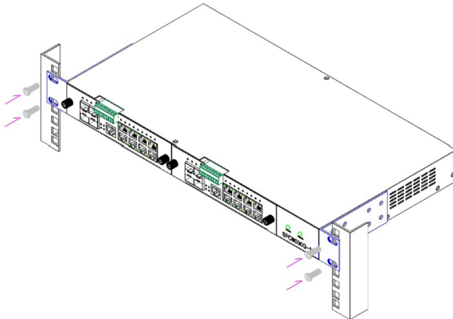
SFC8000G-1U Rack Mount 장착 모습
