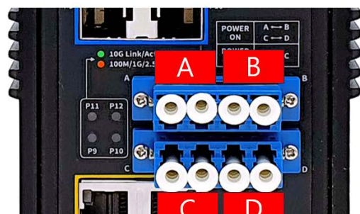
4x4 BYPASS Port
