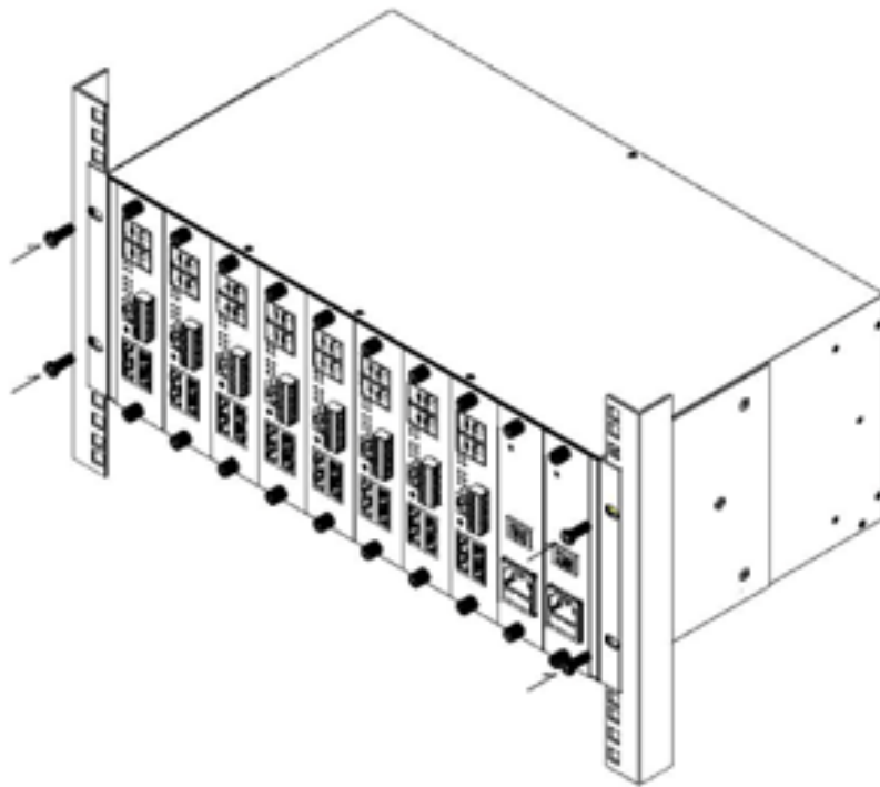
SFC8100G-4U Rack Mount 장착 모습
